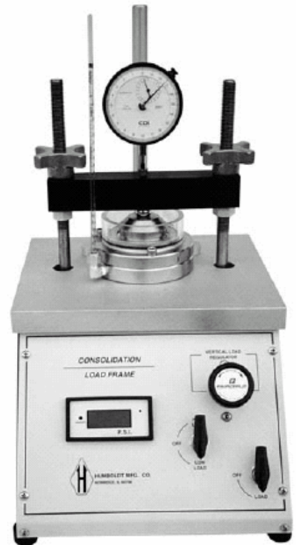
Pneumatic Loading Consolidation Sets for HM-2432, HM-1220 and H-4471CC
